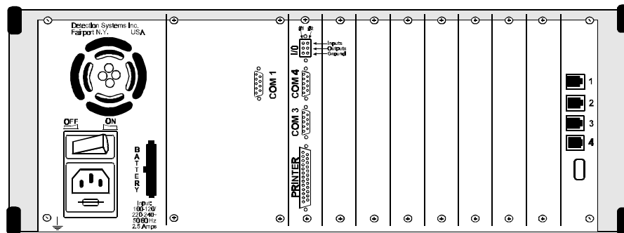
Figure 1-1 D6600 Communications Receiver/Gateway – Rear View
