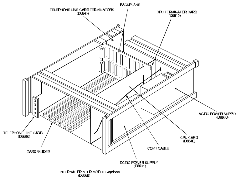
Figure 1-2 Receiver Card Placement
